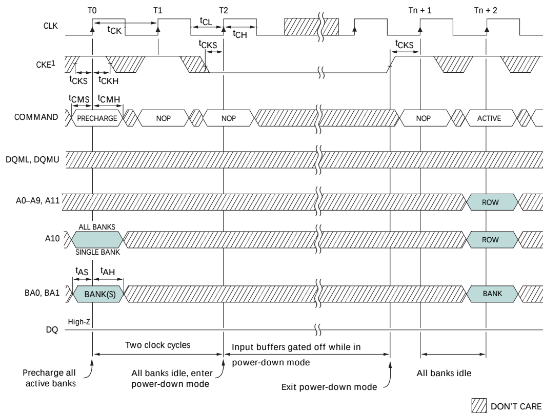
Figure 39: Power-down Mode
