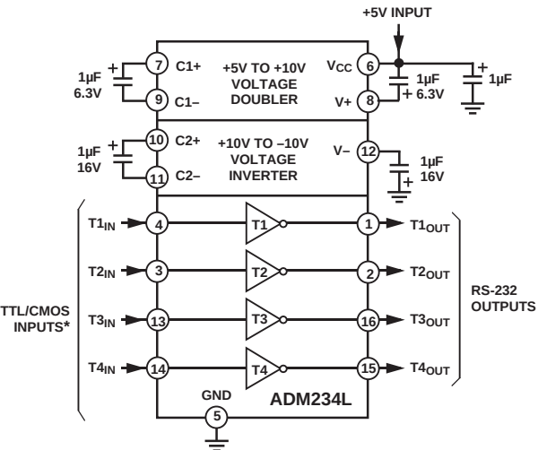
Figure 10. ADM234L Typical Operating Circuit
