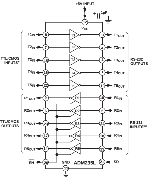
Figure 12. ADM235L Typical Operating Circuit
