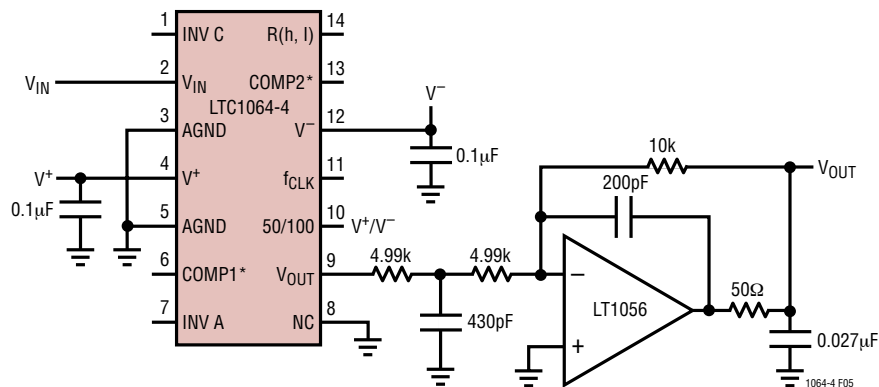
Figure 5. Adding an Output Buffer-Filter to Eliminate Any Clock Feedthrough. Passband Error of Output Buffer is \pm 0.1dB to 50kHz, -3dB at 94kHz.
