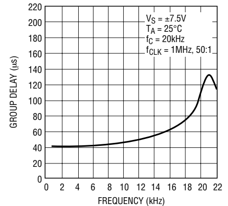
Passband Group Delay
