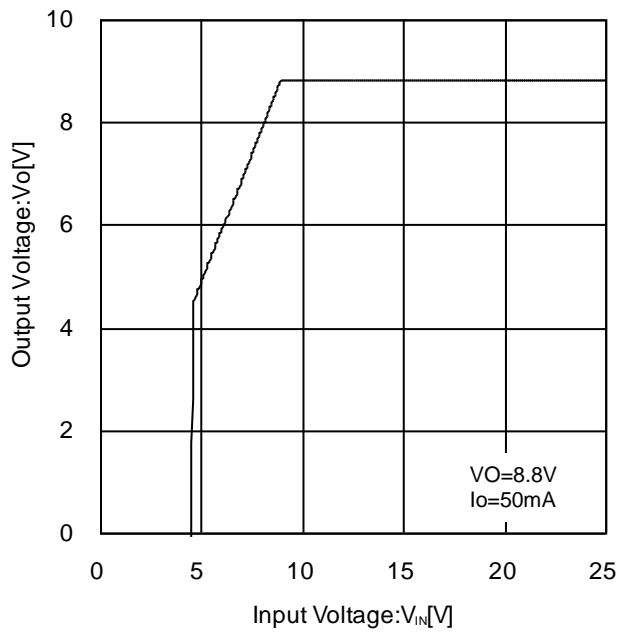
Figure 36. REG2 Output Voltage vs Input Voltage
