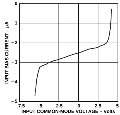
Figure 15. Input Bias Current vs. Input Common-Mode Voltage for \pm 5\text{ V} Supplies
