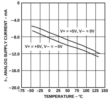
Figure 12. Analog Supply Current vs. Temperature for \pm 5\text{ V} Supplies
