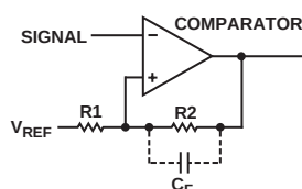
Figure 17. Configuring the AD8598 with Hysteresis
