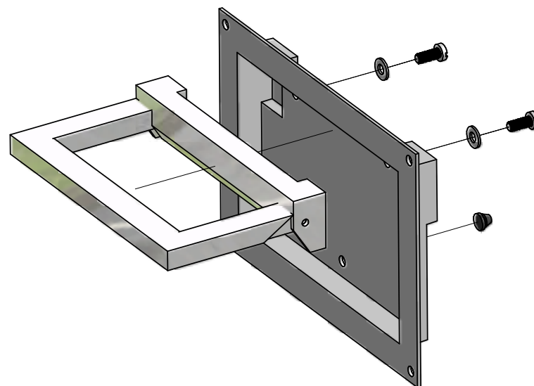
ISO VIEW OF ASSEMBLY
