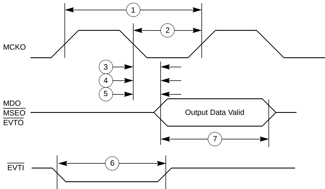
Figure 25. Nexus Timings
