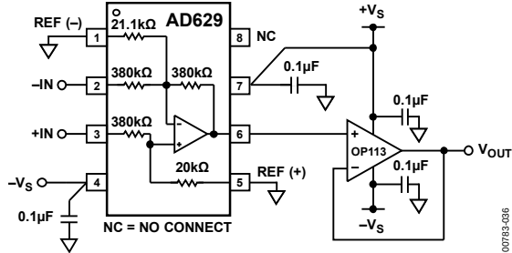
Figure 38. Output Buffering Application
