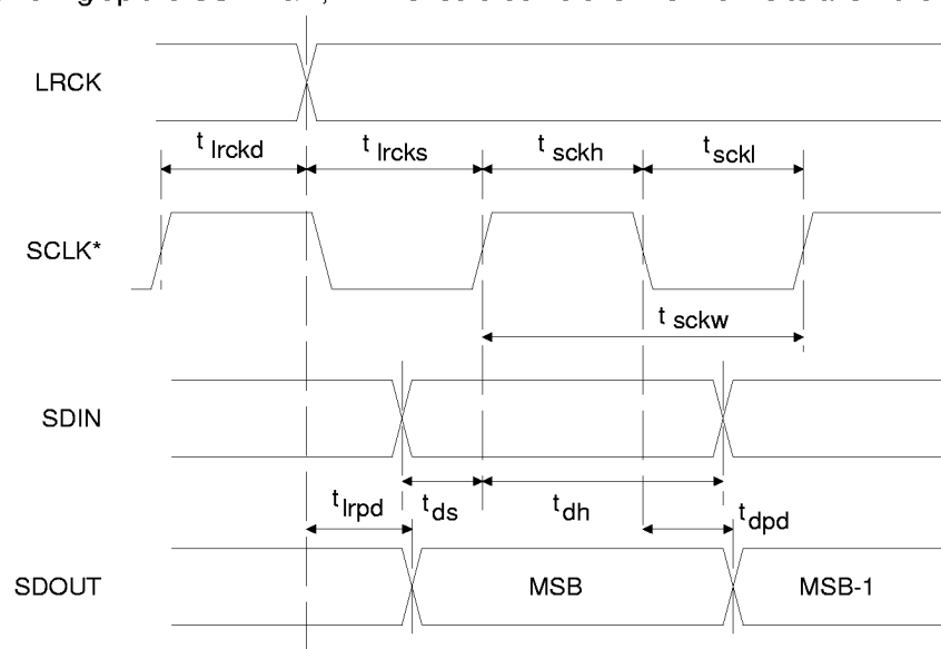
Serial Audio Port Data I/O Timing
