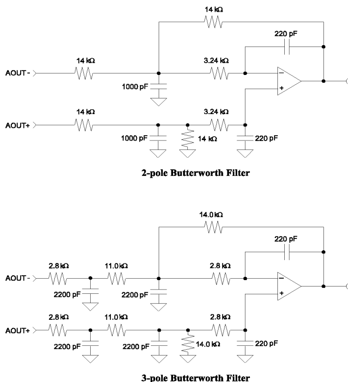
Figure 6. 2- and 3-Pole Butterworth Filters
