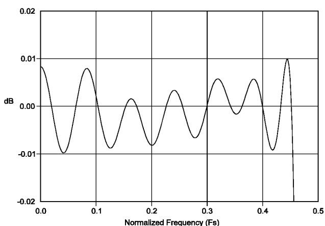
Figure 14. ADC Passband Ripple
