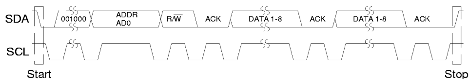
Figure 10. Control Port Timing, I 2 C mode
