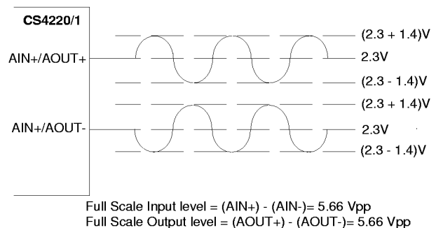
Figure 5. Full Scale Input/Output Voltage
