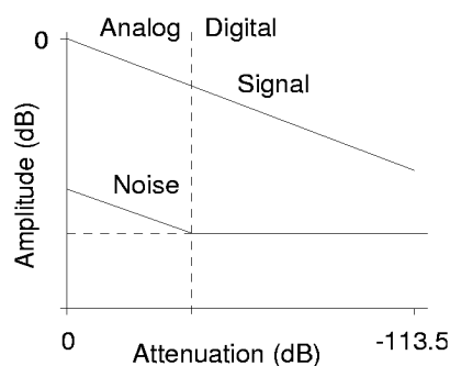
Figure 7. Hybrid Analog/Digital Attenuation
