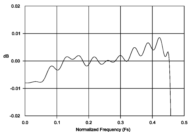
Figure 17. DAC Passband Ripple
