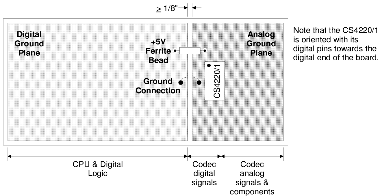
Figure 12. Suggested Layout Guideline (See CDB4220/21 Data Sheet)
