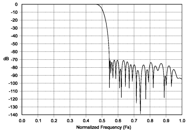
Figure 16. DAC Filter Response
