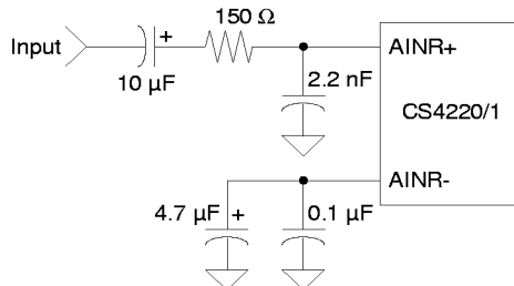
Figure 4. Single-ended Input Application
