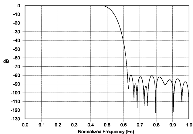
Figure 13. ADC Filter Response
