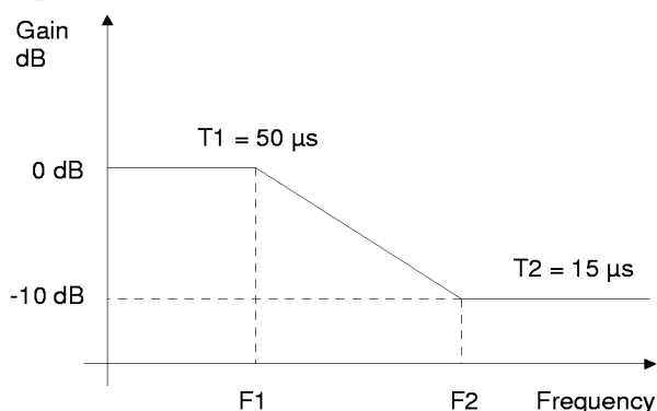
Figure 11. De-emphasis Curve.
