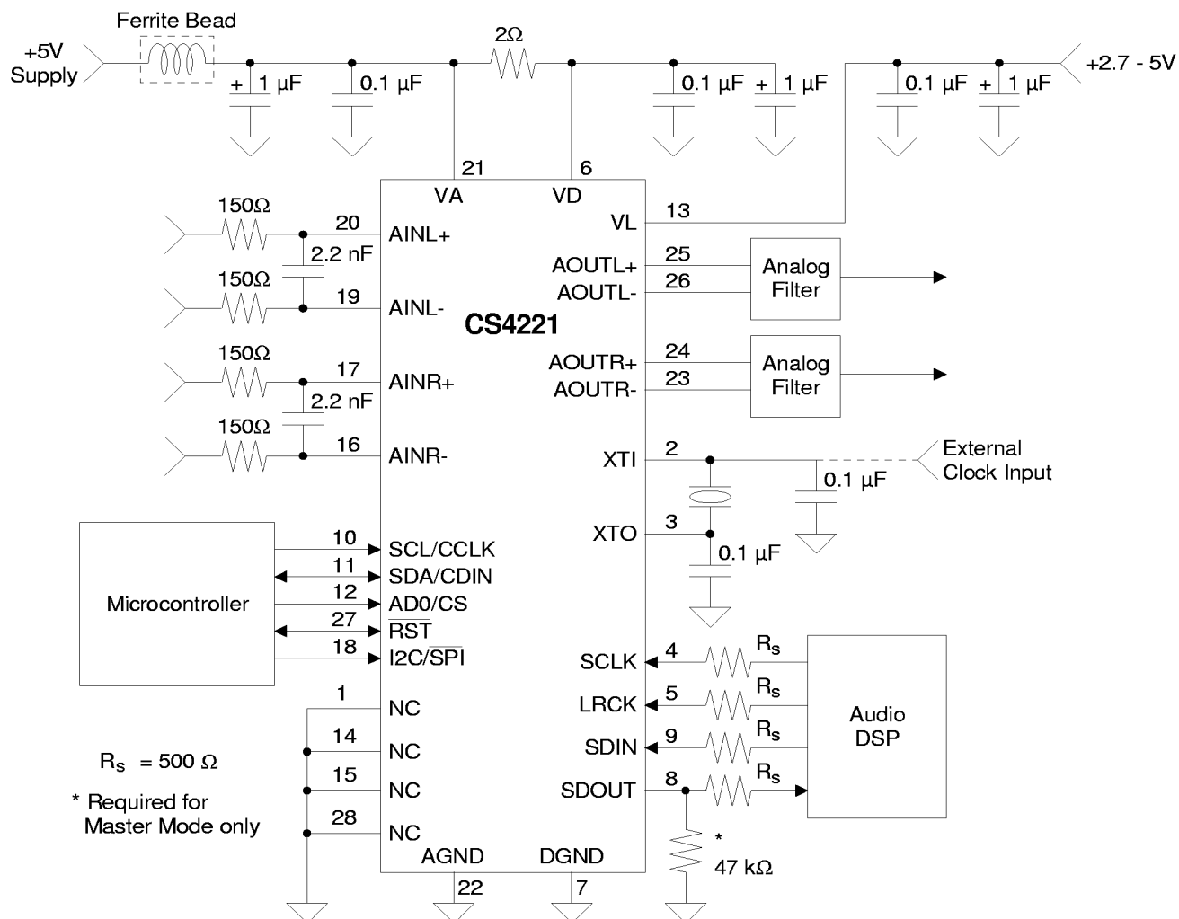
Figure 2. CS4221 Recommended Connection Diagram (Also see Recommended Layout Diagram, Figure 12)
