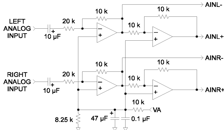
Figure 3. Optional Line Input Buffer
