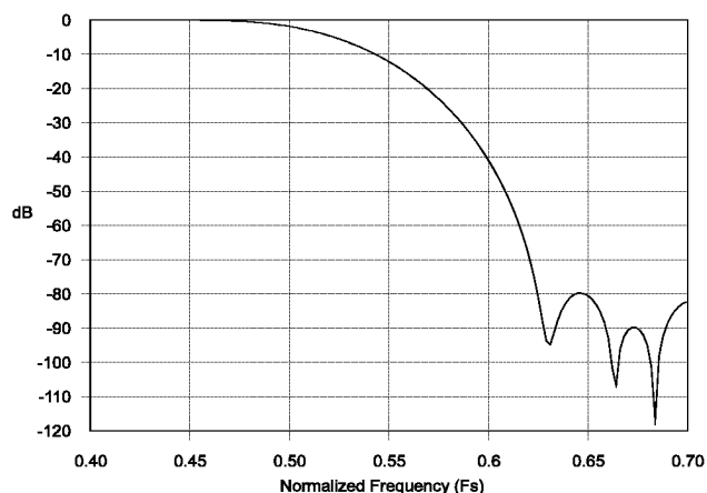
Figure 15. ADC Transition Band
