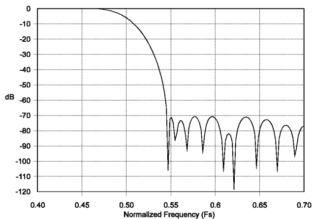
Figure 18. DAC Transition Band
