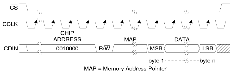
Figure 9. Control Port Timing, SPI mode
