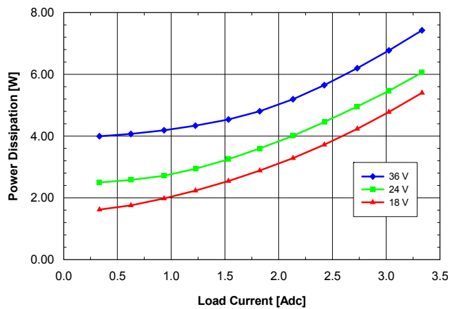
Fig. 7: Power dissipation vs. load current and input voltage for SQ24T/S03150 converter mounted vertically with air flowing from pin 3 to pin 1 at a rate of 300 LFM (1.5 m/s) and T_a = 25\text{ }^{\circ}\text{C} .
