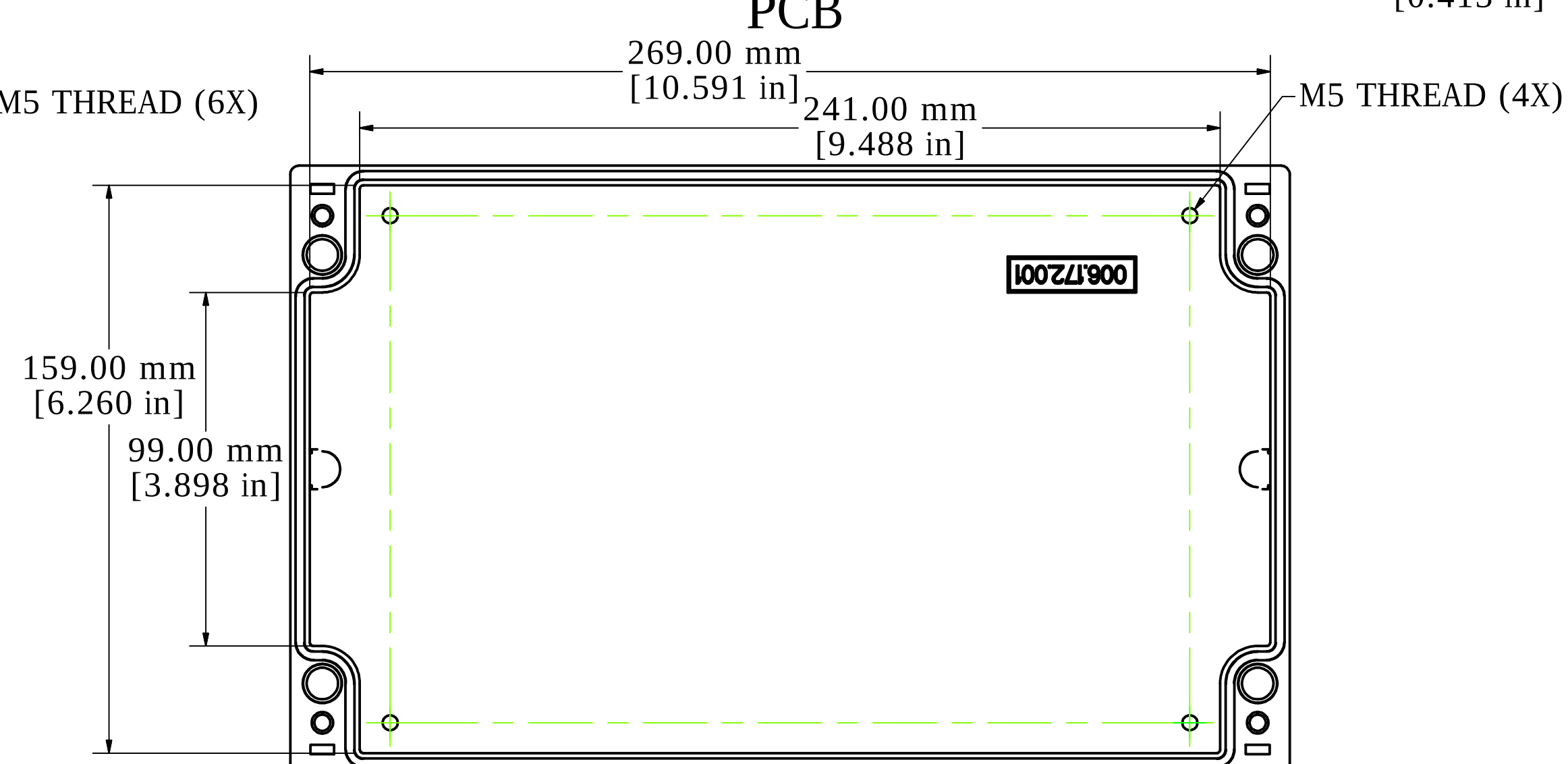
LID - INSIDE VIEW
