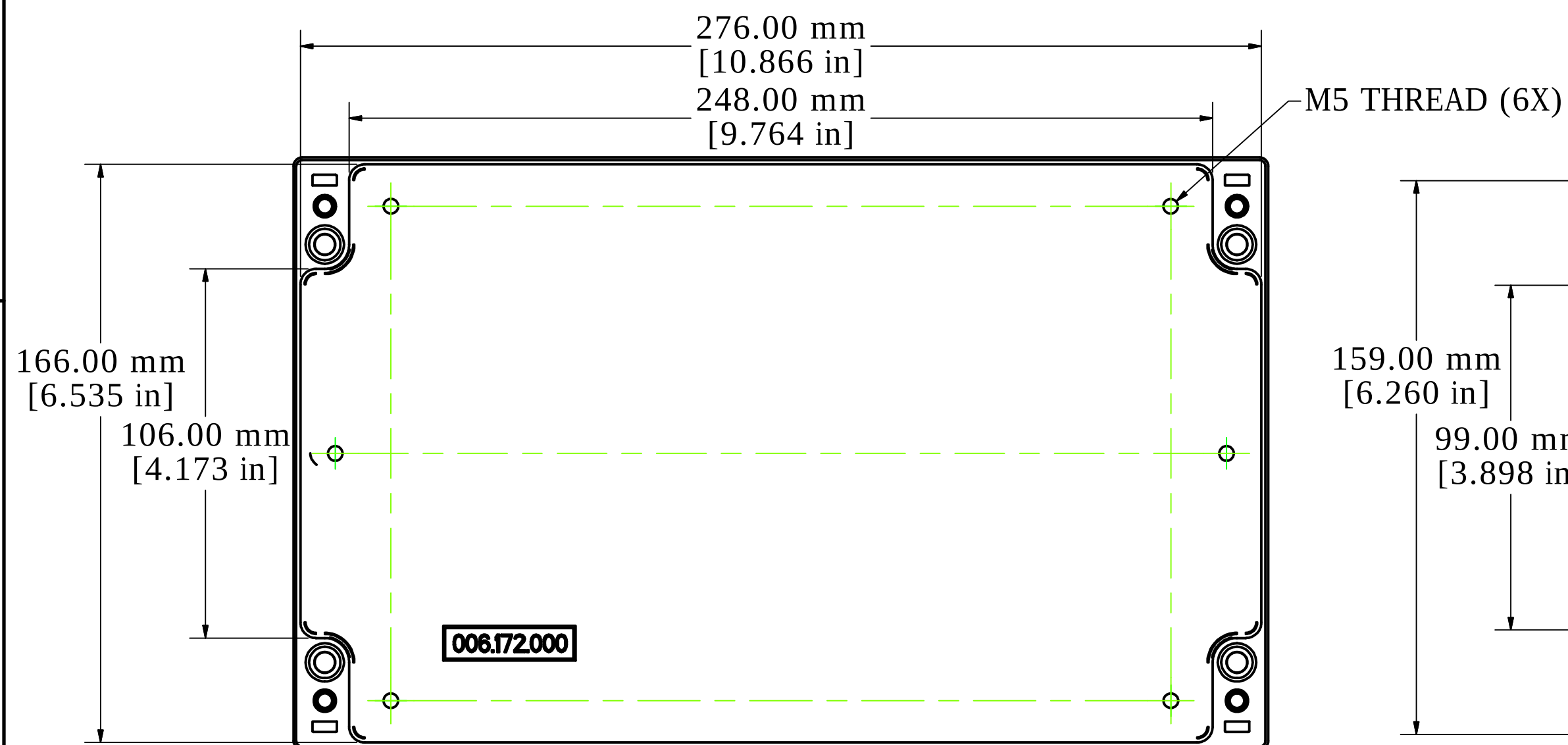
BOX - INSIDE VIEW
