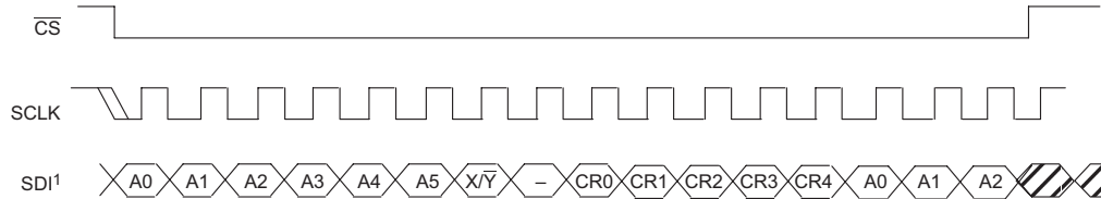
SERIAL PORT WRITE Figure 9
