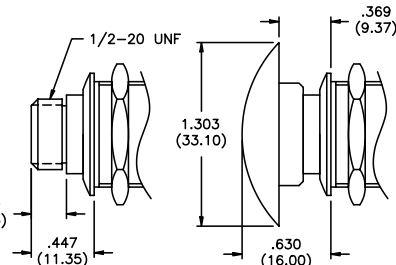
39 threaded Act. & curved bushing
