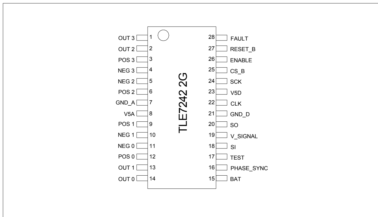
Figure 8 Pin Configuration
