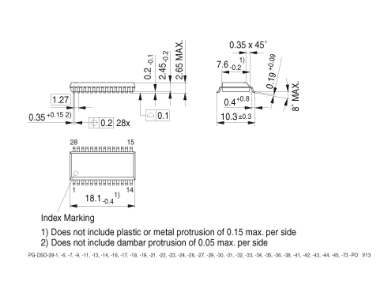
Figure 19 PG-DSO-28
