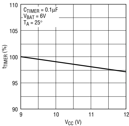
Timer Accuracy vs V_{CC}
