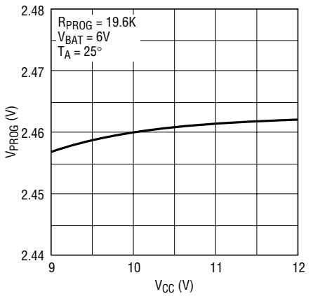
Program Pin Voltage vs V_{CC}
