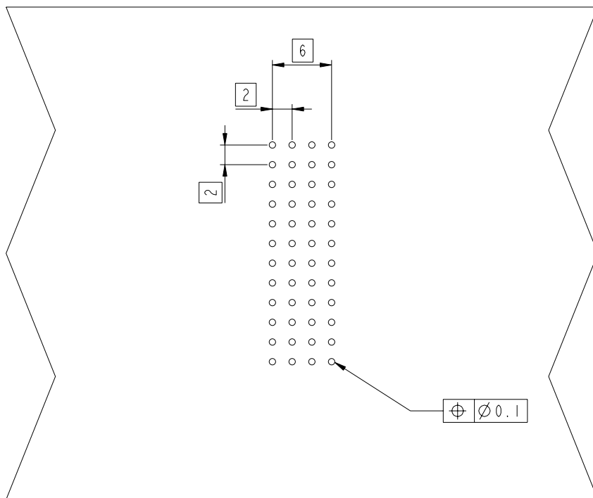
PC BOARD LAYOUT COMPONENT SIDE SCALE 3:1
