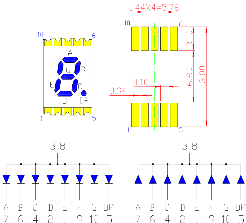
SMA201LB G/W ( Common Anode )
