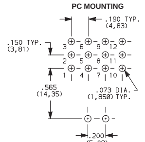
7401MD9AV2BE Vertical Actuation 4PDT
