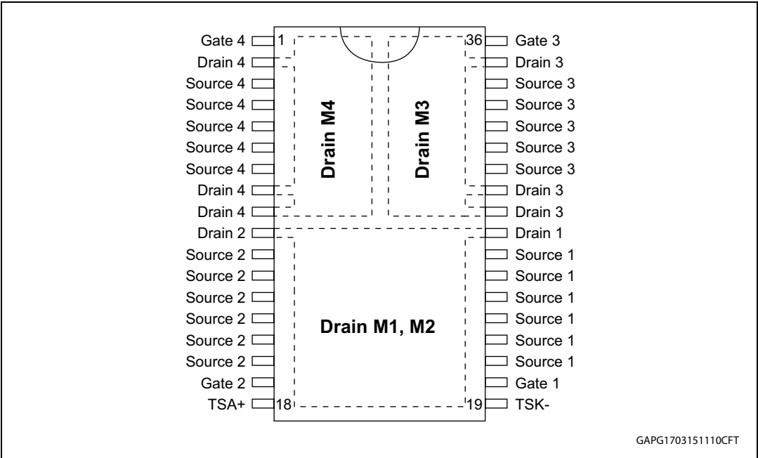
Figure 2. Configuration diagram
