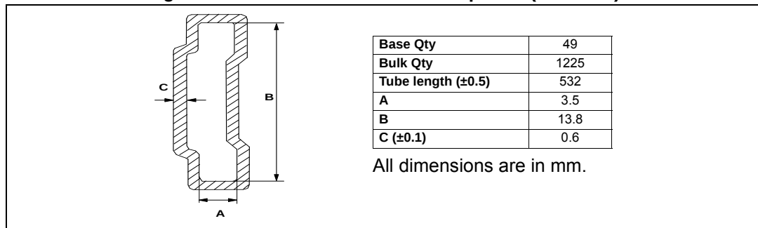
Figure 14. PowerSSO-36 TP tube shipment (no suffix)
