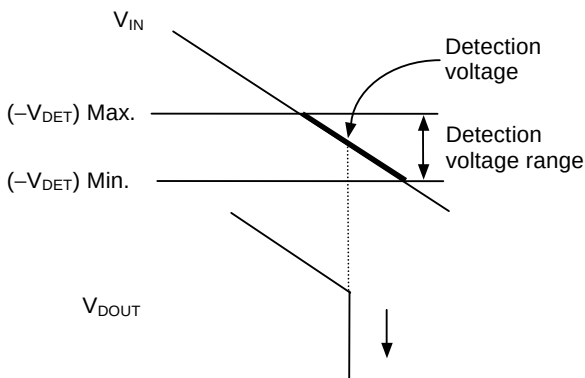
Figure 29 Detection Voltage
