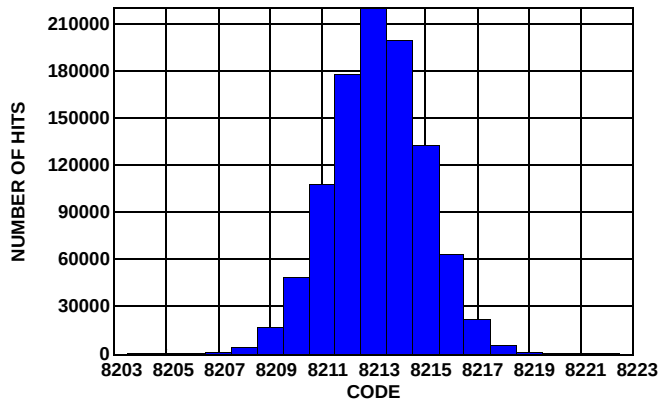
FIGURE 15. NOISE HISTOGRAM
