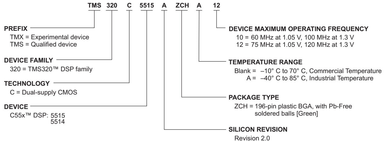
Figure 3-3. Device Nomenclature
