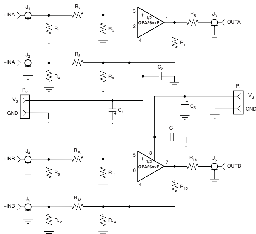
Figure 2. Schematic for DEM-OPA-MSOP-2A
