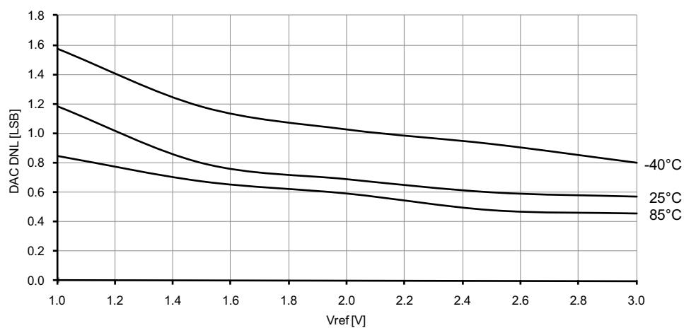
Figure 37-220. DAC DNL error vs. V_{REF} .
