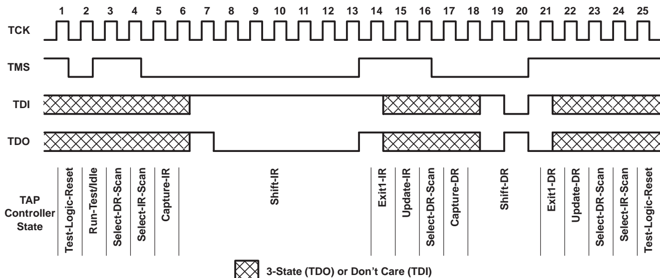
Figure 12. Timing Example
