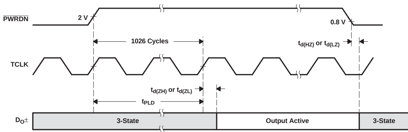
Figure 11. Serializer PLL Lock Time and PWRDN High-Impedance State Delays
