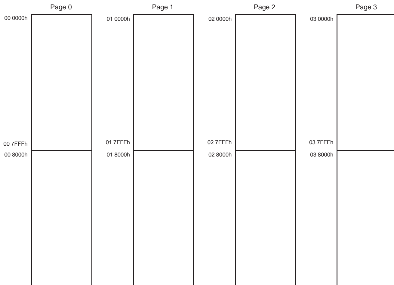
Figure A–3. DMA External Data Memory Map (SLAXS=1, DLAXS=1)
