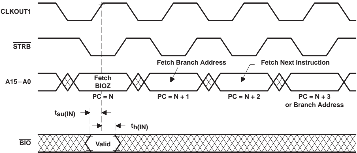
Figure 14. BIO Timing
