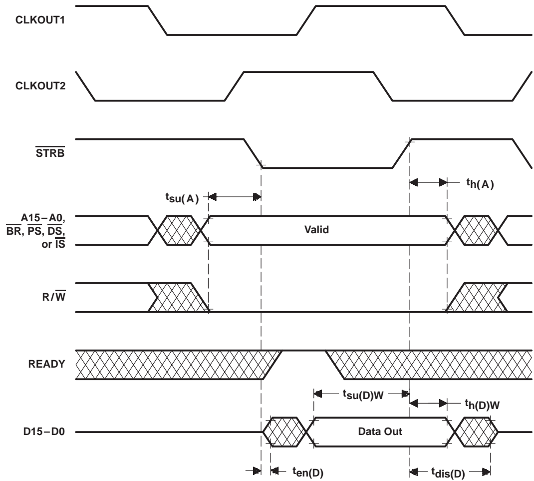
Figure 8. Memory-Write-Cycle Timing
