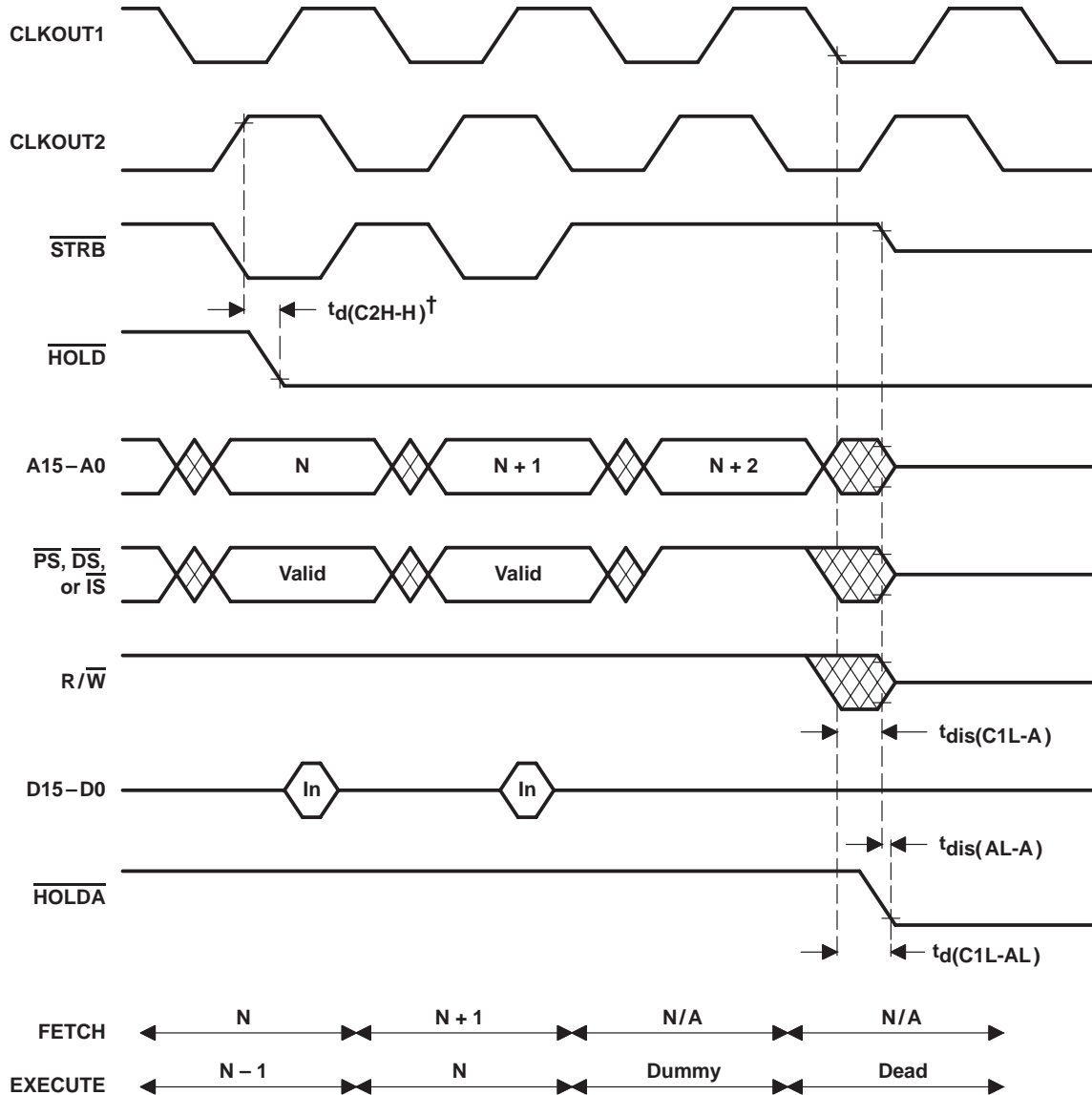
Figure 16. \overline{\text{HOLD}} Timing (Part A)
