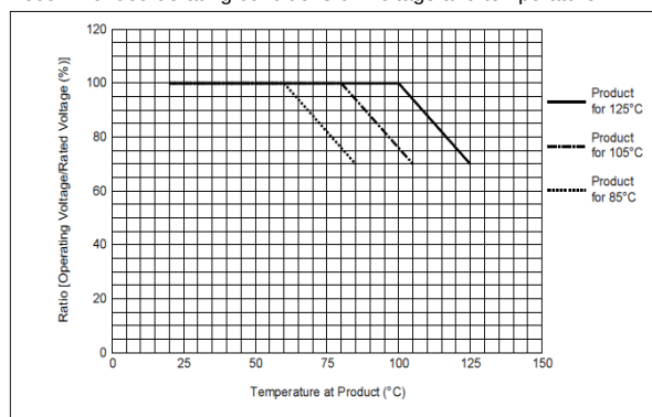
Recommended derating conditions on voltage and temperature
