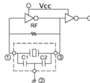
Figure 2) Test Circuit (74HCU04P)
