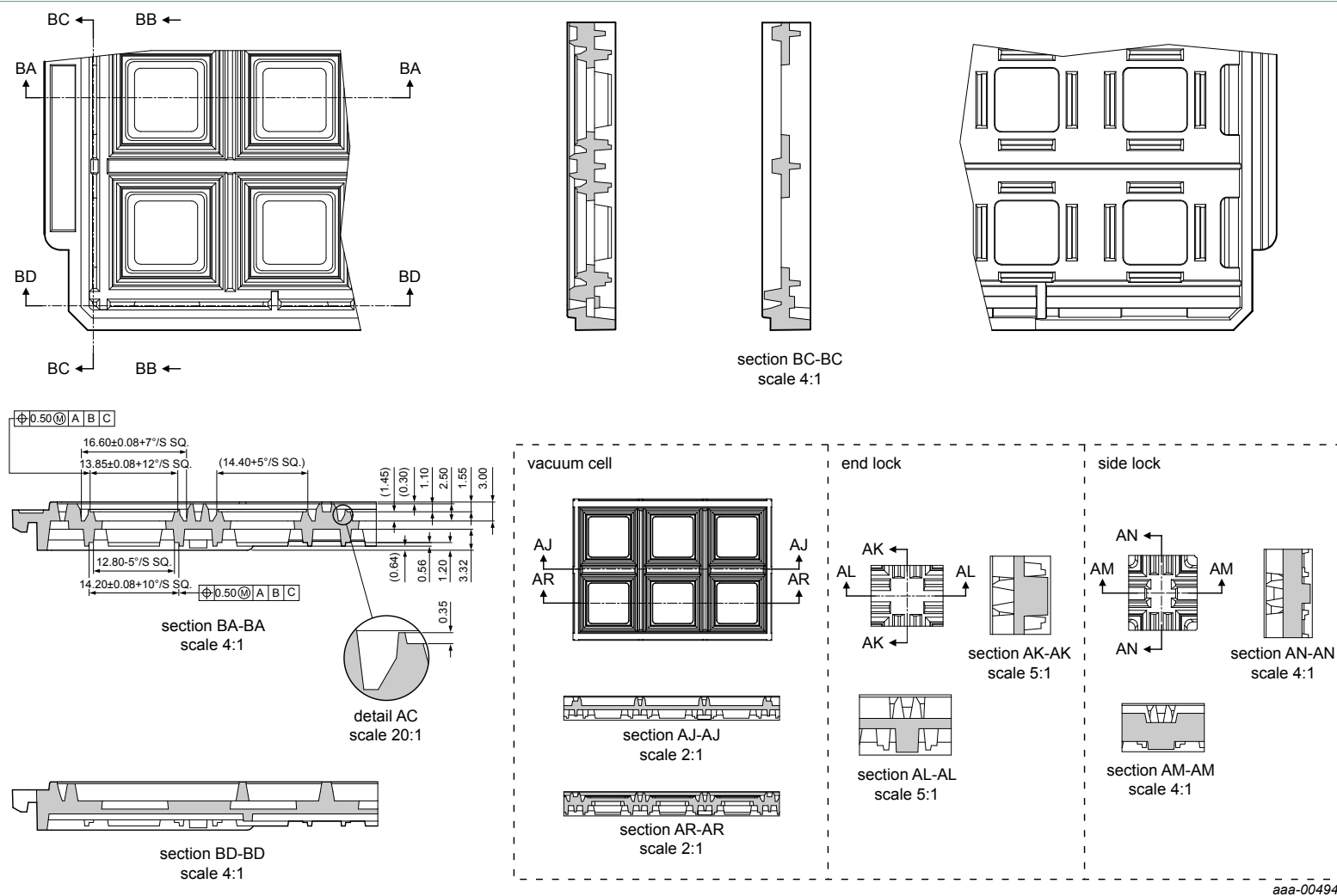
Figure 35. Tray details
