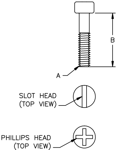
FILLISTER HEAD CAPTIVE SCREW
