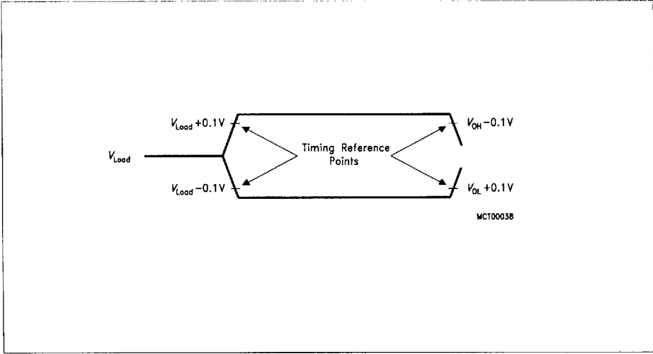
AC Testing: Float Waveforms
