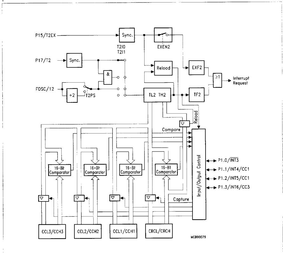
Figure 3 Block Diagram of Timer/Counter 2
