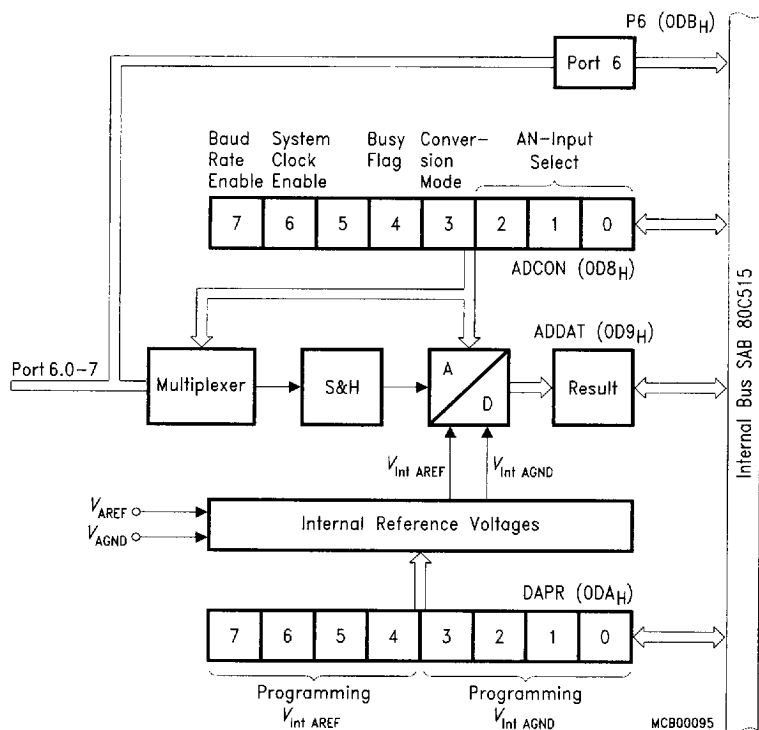
Figure 4 Block Diagram of the A/D Converter
