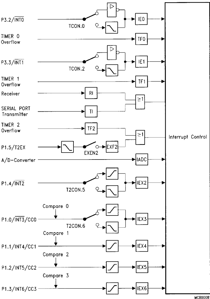
Figure 5 Interrupt Request Sources
