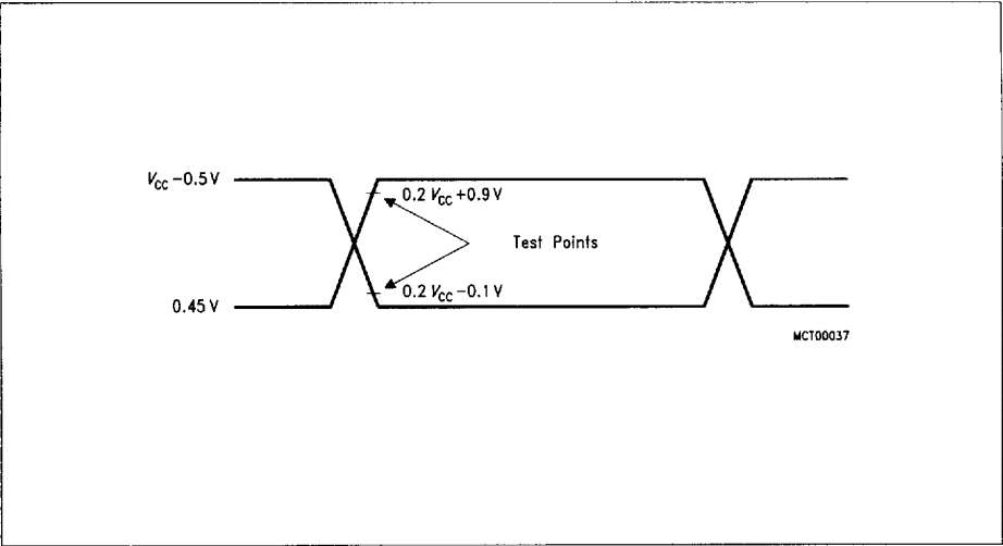
AC Testing: Input, Output Waveforms
