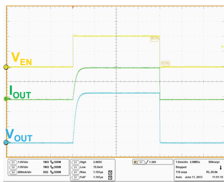
Figure 28. Enable transient
