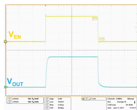
Figure 29. Turn-on time
