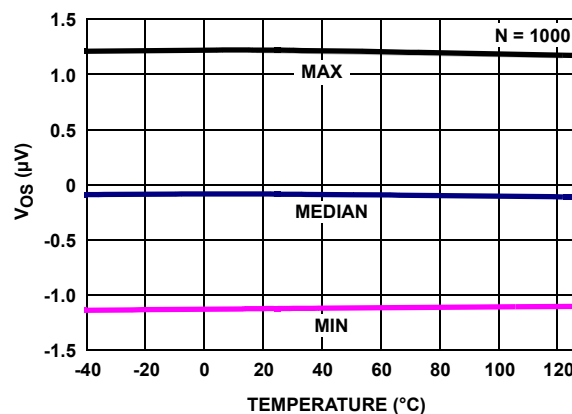
FIGURE 24. V_{OS} (SOT PKG) vs TEMPERATURE, V_{IN} = 0V , V_+ , V_- = \pm 1.2V
