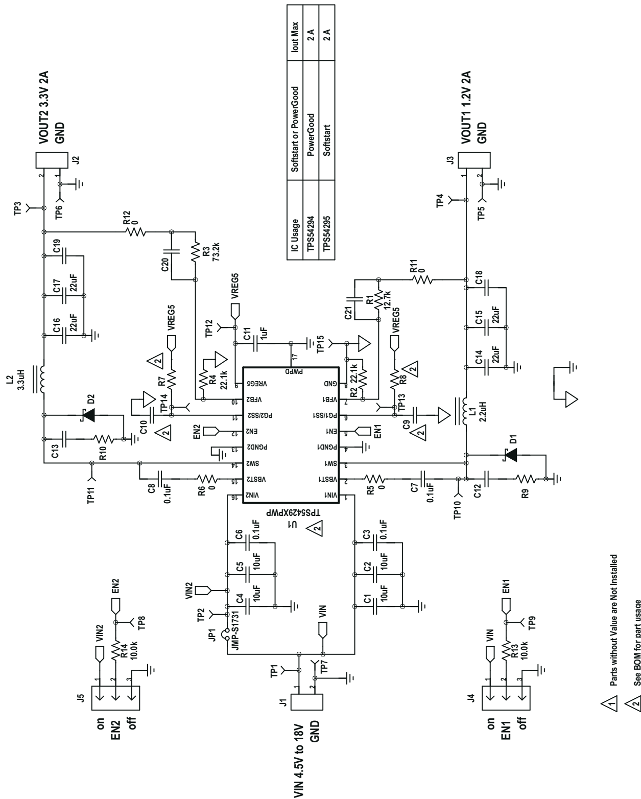
Figure 6-1. TPS54295EVM Schematic Diagram
