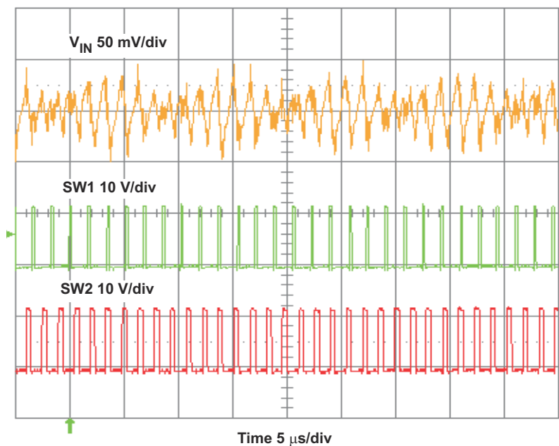
Figure 4-15. TPS54295EVM Input Voltage Ripple
