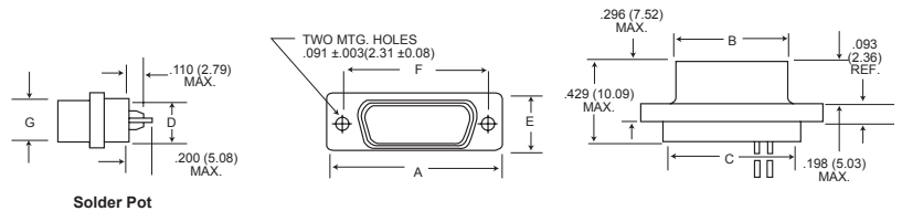
Solder Pot
