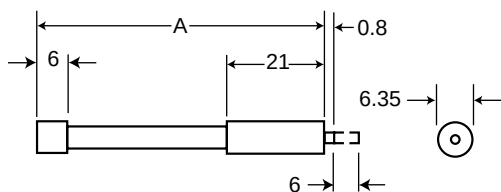
Trip-indicator Fuselink Data
