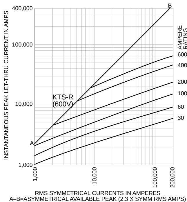
Time-Current Characteristic Curves—Average Melt
