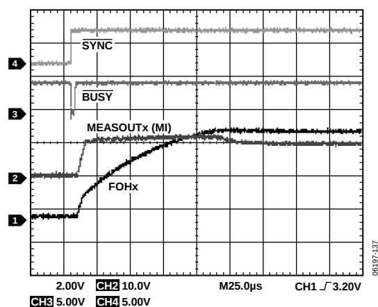
Figure 45. FV Settling, 0 V to 5 V, \pm 20 \mu A Range, C_{LOAD} = 220 pF , CCOMPx = 100 pF , R_{LOAD} = 270 k\Omega
