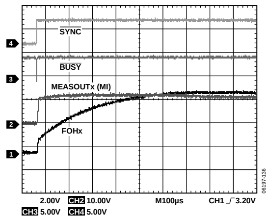
Figure 44. FV Settling, 0 V to 5 V, \pm 5 \mu A Range, C_{LOAD} = 220 pF , CCOMPx = 100 pF , R_{LOAD} = 1 M\Omega
