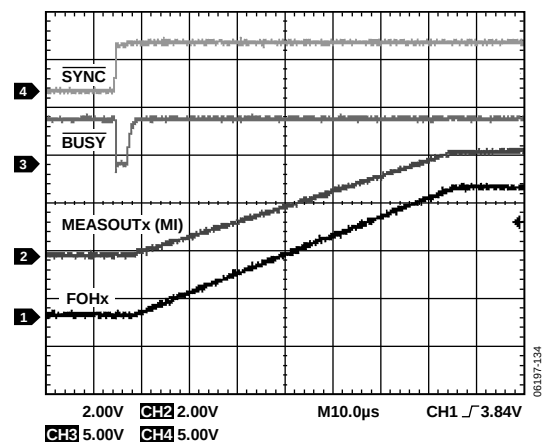
Figure 42. FV Settling, 0 V to 5 V, \pm 2 mA Range, C_{LOAD} = 220 pF , CCOMPx = 1 nF , R_{LOAD} = 5.6 k\Omega
