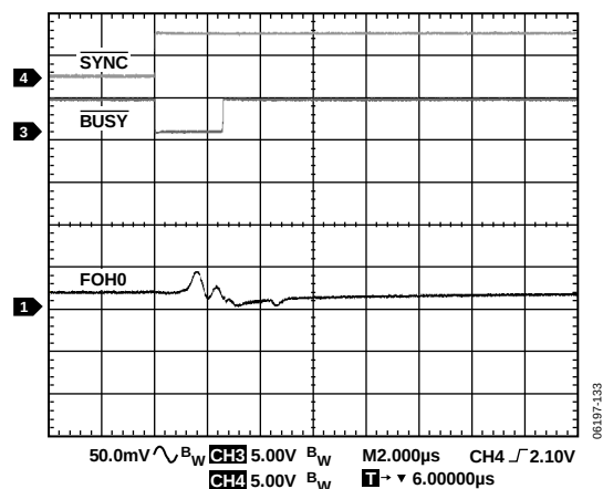
Figure 41. Range Change, PMU0, \pm 2 mA to \pm 20 \mu A , C_{LOAD} = 1 nF , R_{LOAD} = 150 k\Omega , FV = 3 V
