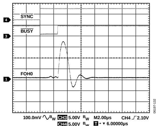
Figure 40. Range Change, PMU0, \pm 20 \mu A to \pm 2 mA , C_{LOAD} = 1 nF , R_{LOAD} = 150 k\Omega , FV = 3 V
