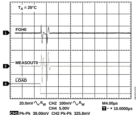
Figure 31. AC Crosstalk, FVMI Mode, PMU 0, Full-Scale Transition on One CPH DAC, MI Gain = 10, MEASOUT Gain = 1, \pm 2 mA Range, C_{LOAD} = 200 pF
