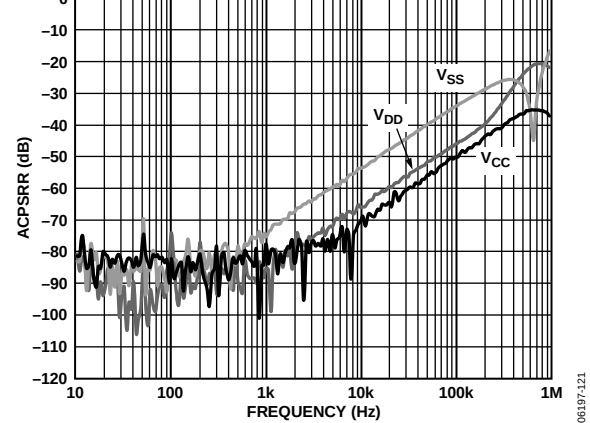
Figure 27. ACPSRR at MEASOUTx in Measure Current Mode vs. Frequency (MI Gain = 5, MEASOUT Gain = 1)
