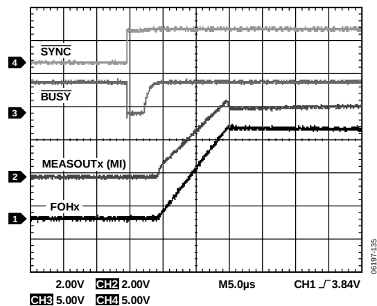
Figure 43. FV Settling, 0 V to 5 V, \pm 2 mA Range, C_{LOAD} = 220 pF , CCOMPx = 100 pF , R_{LOAD} = 5.6 k\Omega
