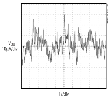
MAX6165 NOISE
