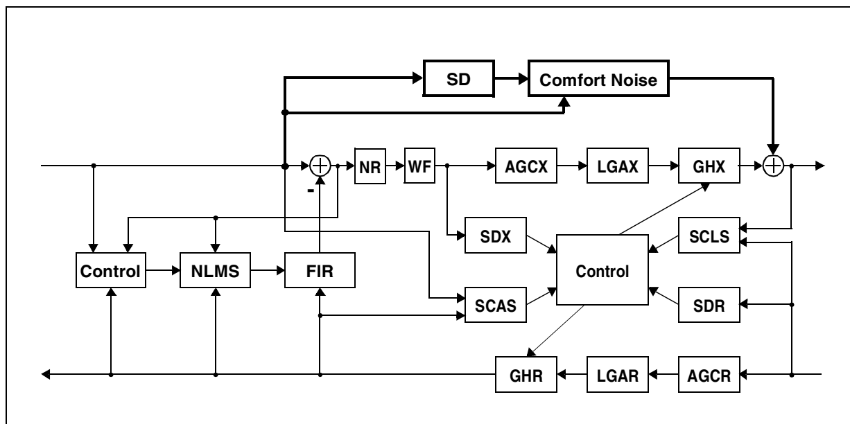
Figure 26 Comfort Noise Generator - Integration into Speakerphone
