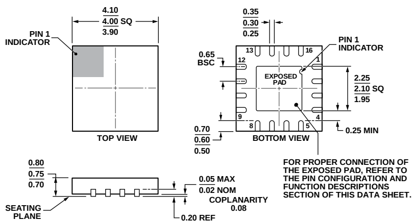
Figure 53. 16-Lead Lead Frame Chip Scale Package [LFCSP_WQ] 4 mm x 4 mm Body, Very Thin Quad (CP-16-23) Dimensions shown in millimeters
