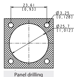
Panel drilling
