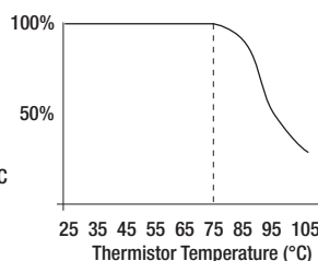
LED Current
