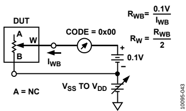
Figure 34. Wiper Resistance
