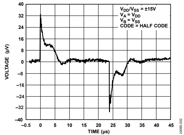
Figure 27. Digital Feedthrough
