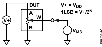
Figure 33. Potentiometer Divider Nonlinearity Error (INL, DNL)
