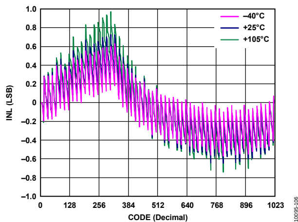
Figure 6. R-INL in R-Perf Mode vs. Code
