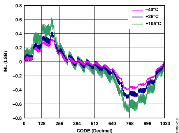
Figure 12. INL in Normal Mode vs. Code
