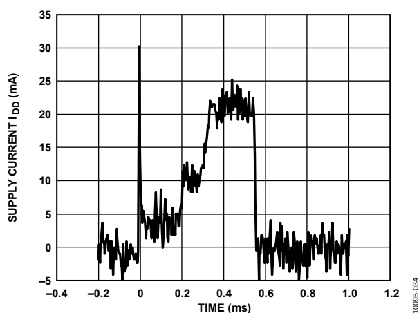
Figure 23. I_{DD} Waveform While Blowing/Reading Fuse
