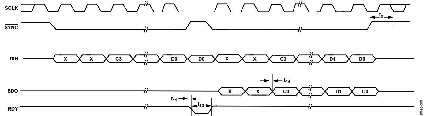
Figure 4. Read Timing Diagram, CPOL = 0, CPHA = 1
