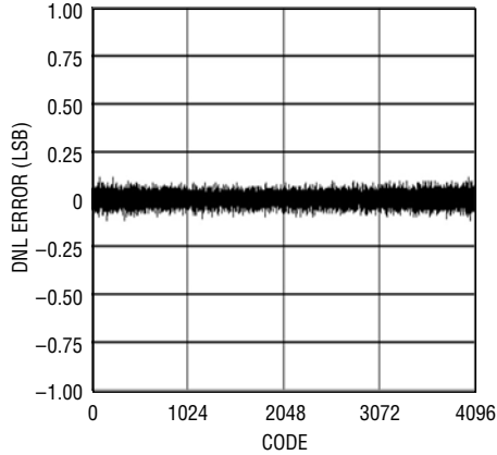
LTC2292: Typical DNL, 2V Range, 40Msps
