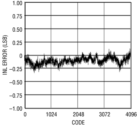
LTC2292: Typical INL, 2V Range, 40Msps
