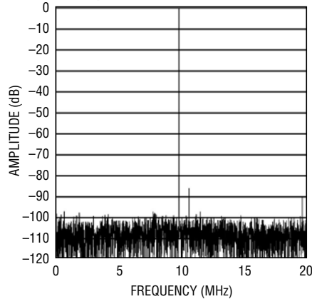
LTC2292: 8192 Point FFT, f_{IN} = 70\text{MHz} , -1dB, 2V Range, 40Msps
