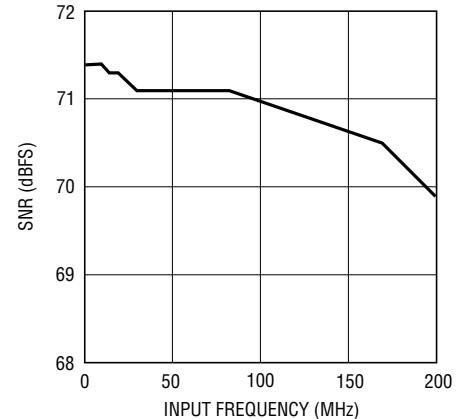
LTC2292: SNR vs Input Frequency, -1dB, 2V Range, 40Msps
