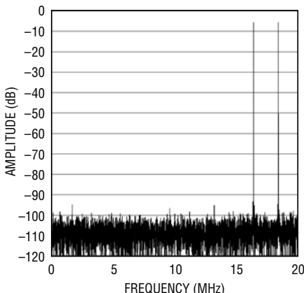
LTC2292: 8192 Point 2-Tone FFT, f_{IN} = 21.6\text{MHz} and 23.6\text{MHz} , -1dB, 2V Range, 40Msps
