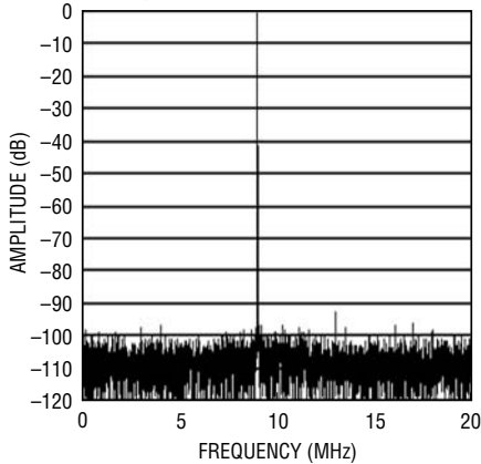
LTC2292: 8192 Point FFT, f_{IN} = 30\text{MHz} , -1dB, 2V Range, 40Msps
