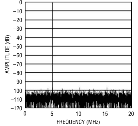
LTC2292: 8192 Point FFT, f_{IN} = 5\text{MHz} , -1dB, 2V Range, 40Msps
