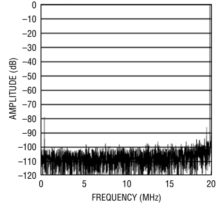
LTC2292: 8192 Point FFT, f_{IN} = 140\text{MHz} , -1dB, 2V Range, 40Msps
