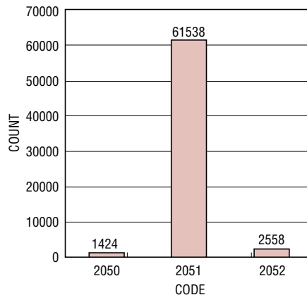
LTC2292: Grounded Input Histogram, 40Msps
