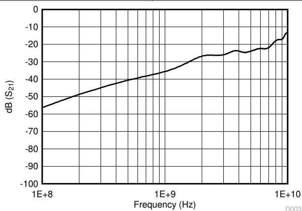
Figure 6-3. Off Isolation
