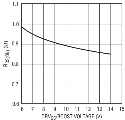
Driver Pull-Down R_{\text{DS(ON)}} vs Supply Voltage
