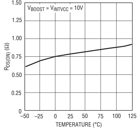
Driver Pull-Down R_{\text{DS(ON)}} vs Temperature
