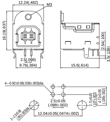
Type B With upper flange <Through-hole type>
