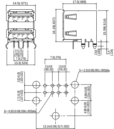
Type A Double-stack
