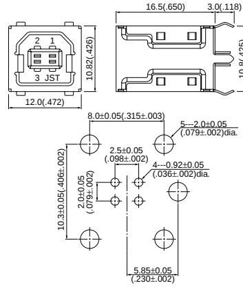
Type B Straight <Through-hole type>
