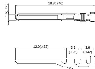
Contact (Crimp type)
