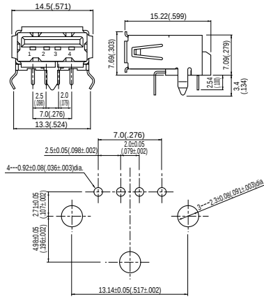
Type A Normal
