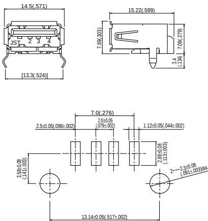
Type A Without flange
