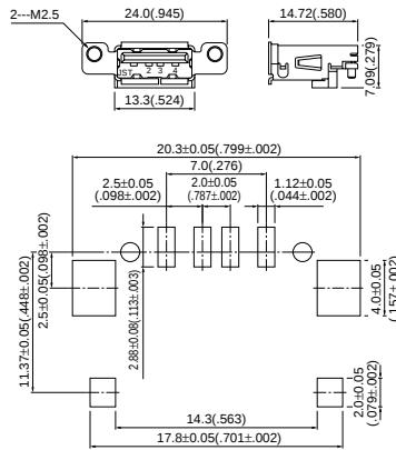
Type A With side flange <SMT type, off-set 3mm (.118")>
