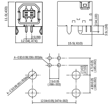
Type B Normal <Through-hole type>
