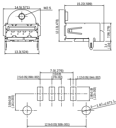
Type A With upper flange
