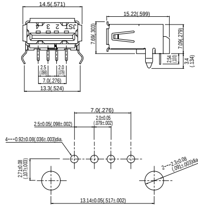
Type A Reverse
