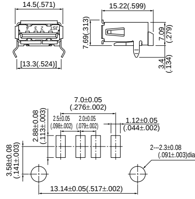
Type A Reverse <SMT type>
