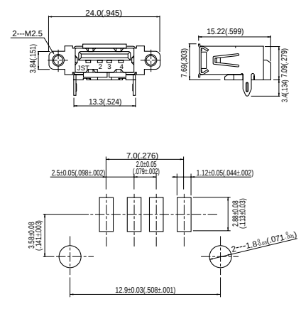
Type A With side flange
