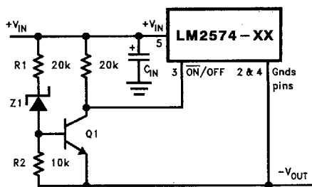
FIGURE 13. Undervoltage Lockout for Buck Circuit
