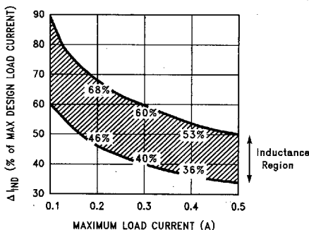
FIGURE 10. Inductor Ripple Current ( \Delta I_{\text{IND}} ) Range Based on Selection Guides from Figures 4-8 .
