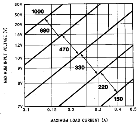
FIGURE 5. LM2574HV-5.0 Inductor Selection Guide
