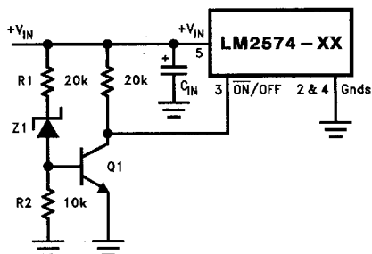
FIGURE 13. Undervoltage Lockout for Buck Circuit
