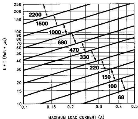
FIGURE 8. LM2574HV-ADJ Inductor Selection Guide
