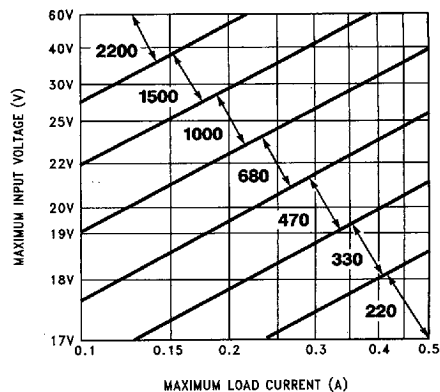
FIGURE 7. LM2574HV-15 Inductor Selection Guide
