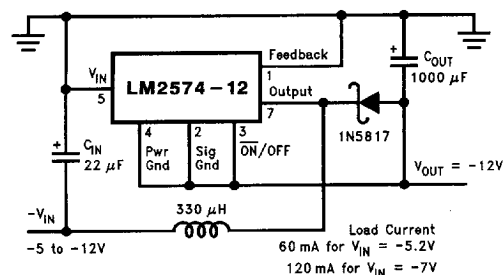
FIGURE 12. Negative Boost
