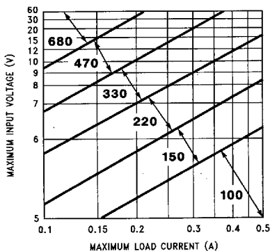
FIGURE 4. LM2574HV-3.3 Inductor Selection Guide
